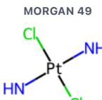
MORGAN 49
