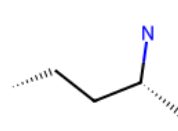
MORGAN 82
