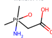
MORGAN 148
