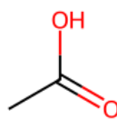
MORGAN 89
