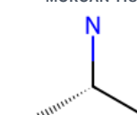
MORGAN 118
