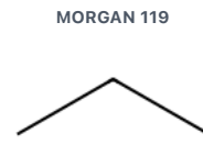
MORGAN 119
