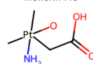
MORGAN 148
