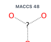
MACCS 48
