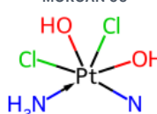
MORGAN 95
