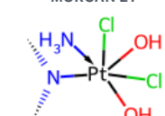
MORGAN 21
