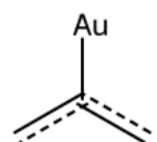
Morgan 152
