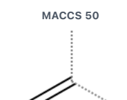
MACCS 50
